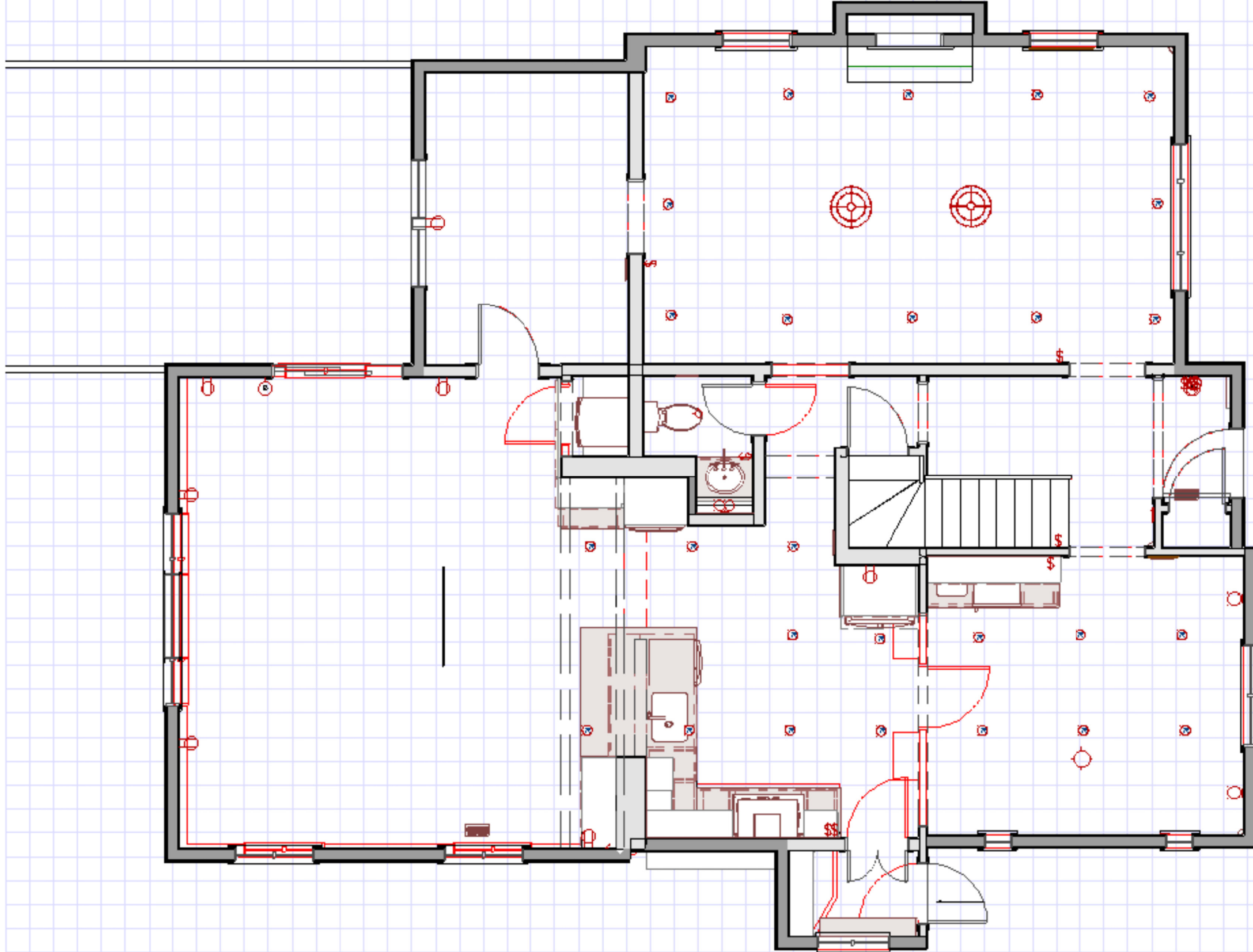
AS BUILT MASK PLAN VIEW
