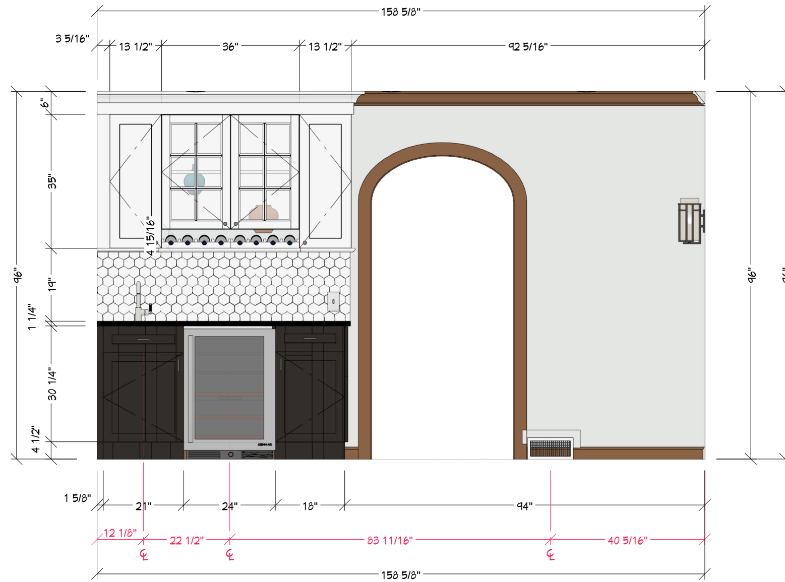
Elevation 15 -Bar Cabinet
